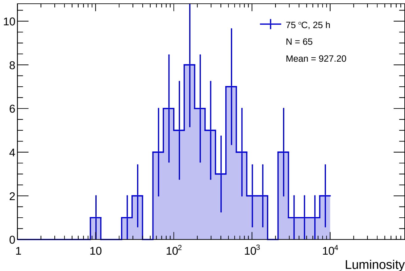
Sensor B1 - 75 °C, 25 h luminosity distribution
