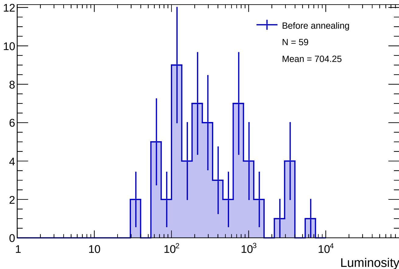
Sensor B1 - Before annealing luminosity distribution
