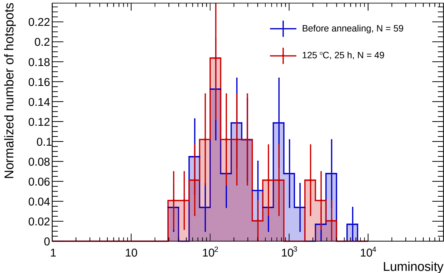
Sensor B1 - Before annealing vs 125 °C, 25 h luminosity distributions
