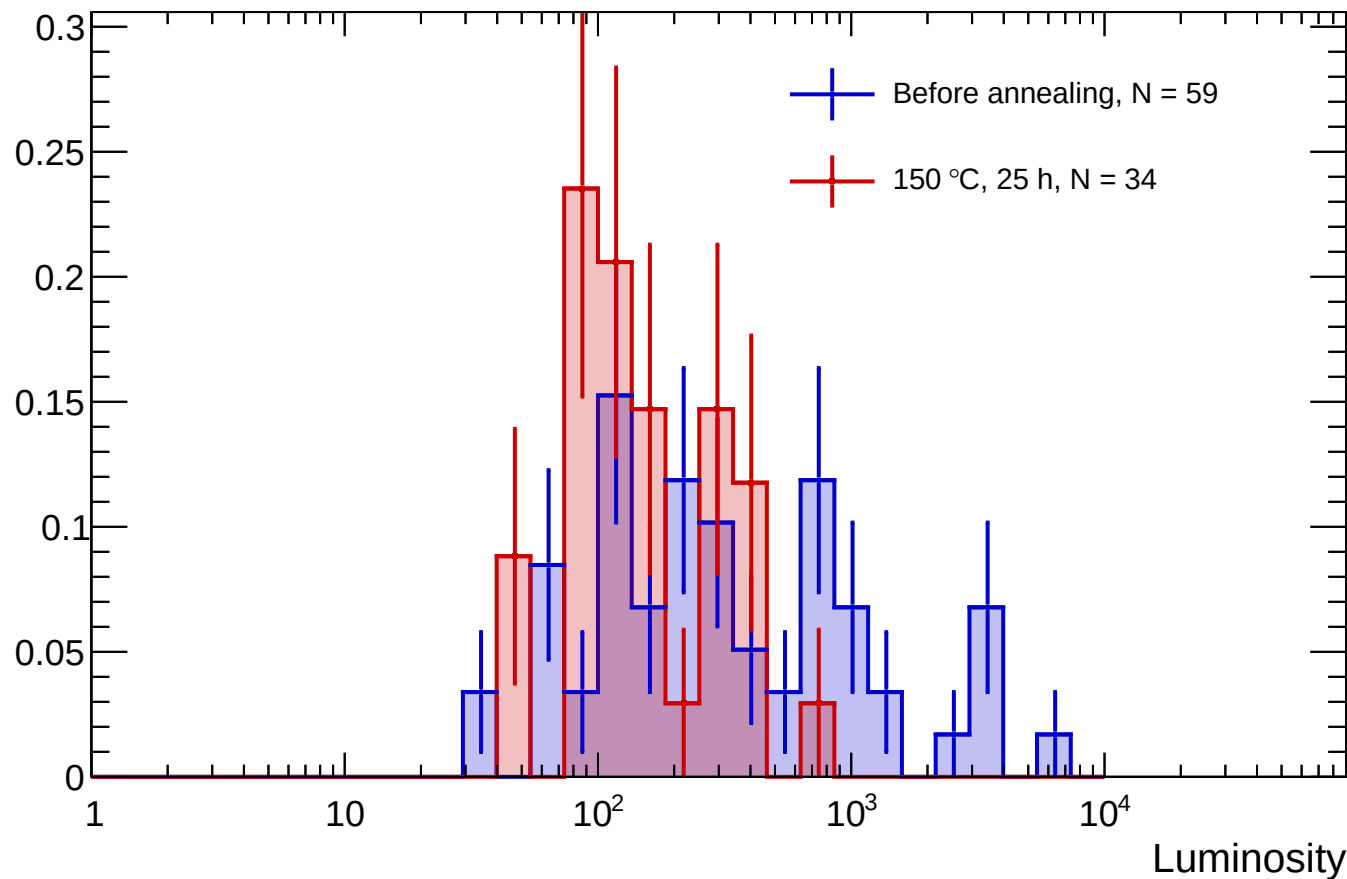
Sensor B1 - Before annealing vs 150 °C, 25 h luminosity distributions
