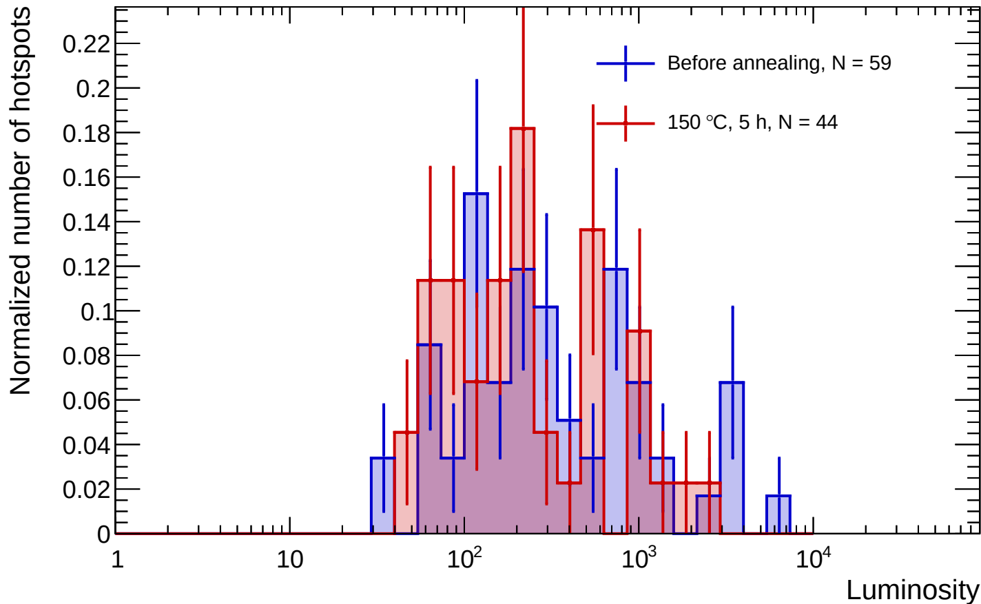
Sensor B1 - Before annealing vs 150 °C, 5 h luminosity distributions
