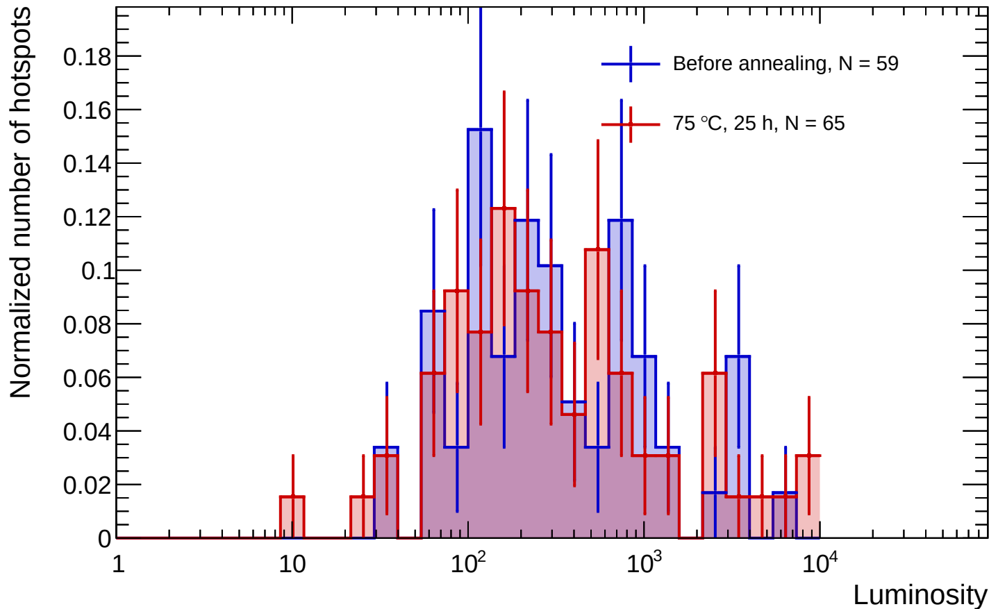
Sensor B1 - Before annealing vs 75 °C, 25 h luminosity distributions
