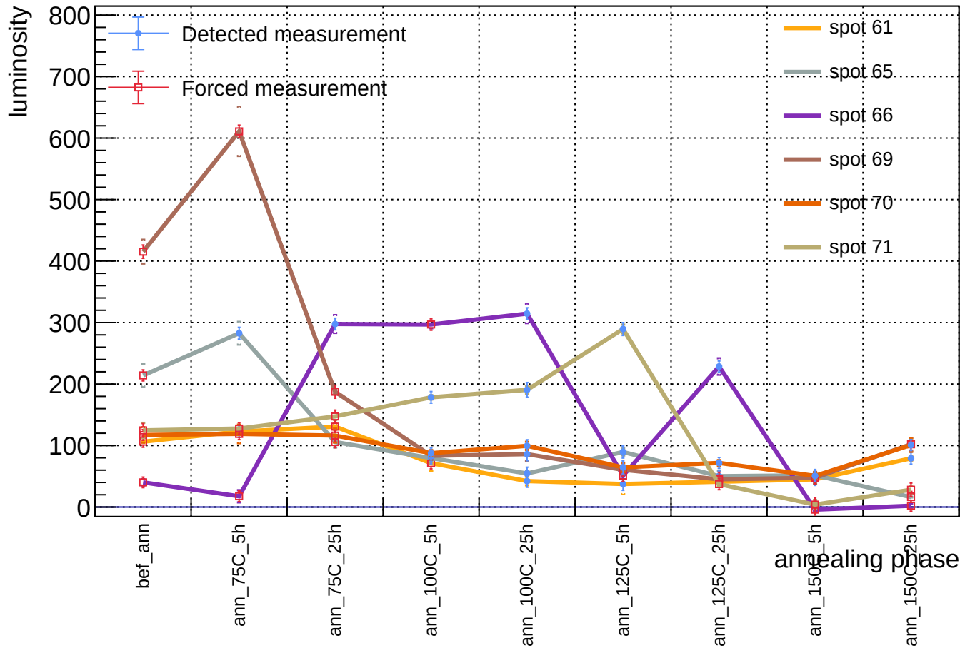
Sensor A1, T = 20 C, representative v = 58.3 V (max available) - luminosity vs phase - order 10^2
