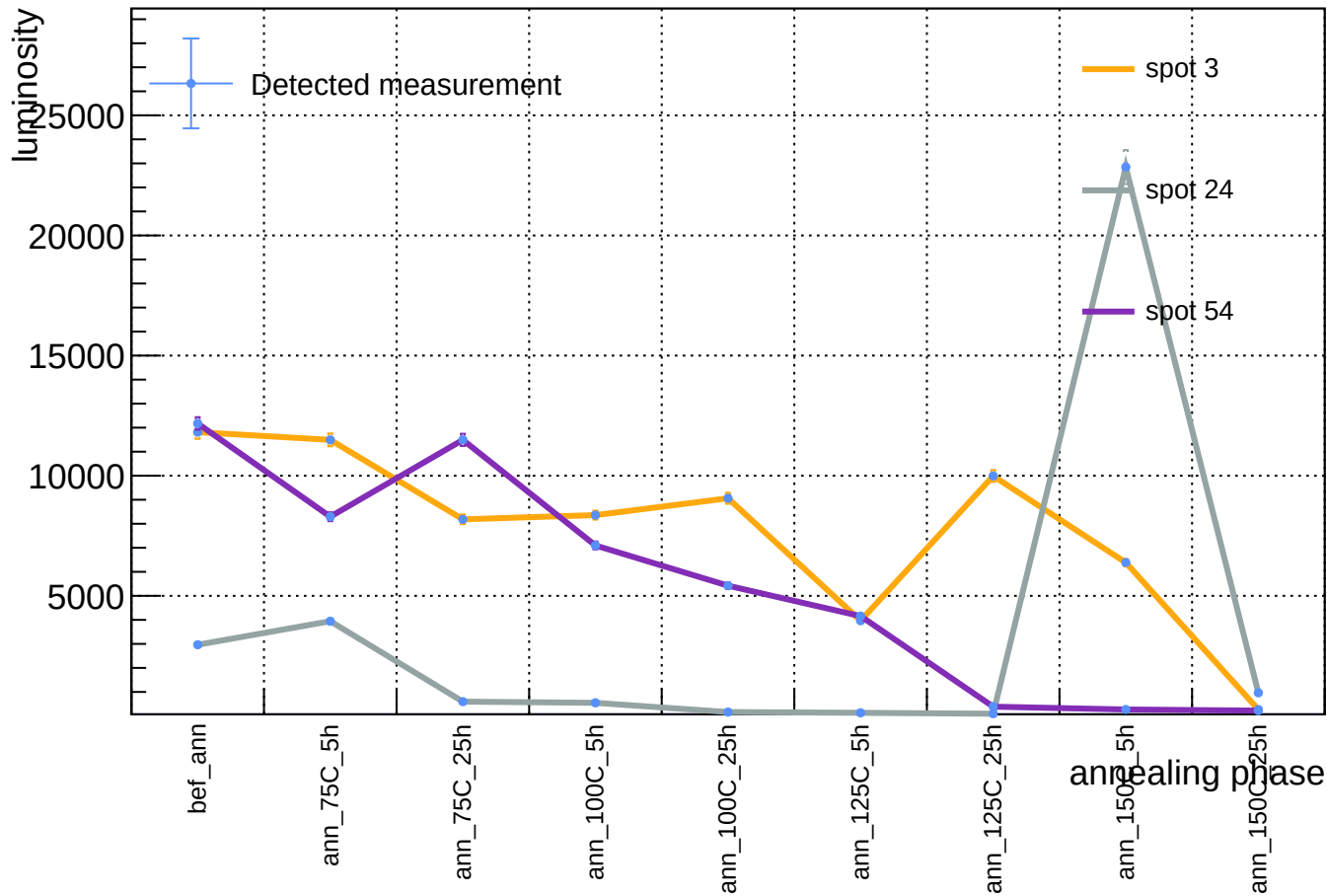
Sensor A1, T = 20 C, representative v = 58.3 V (max available) - luminosity vs phase - order 10 4
