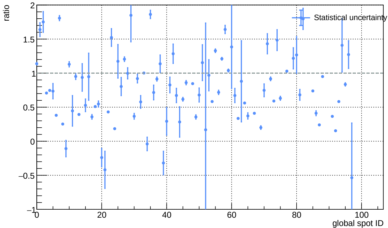
Sensor A1, T = 20 C - L(\text{ann\_100C\_5h}) / L(\text{before\_annealing})
