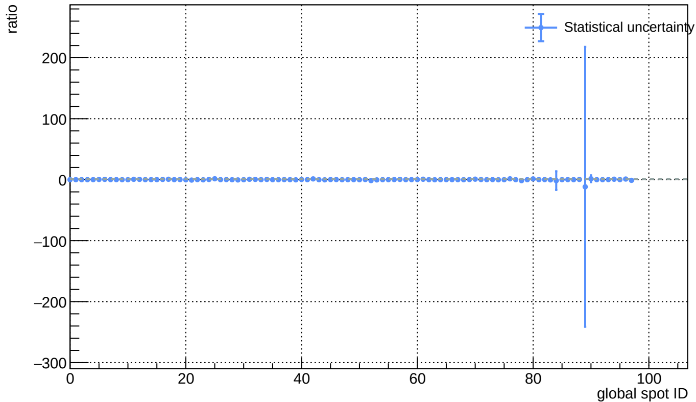
Sensor A1, T = 20 C - L(ann_150C_25h) / L(before_annealing)
