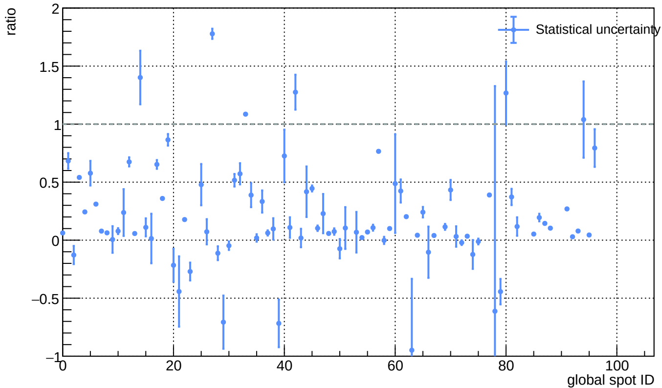
Sensor A1, T = 20 C - L(\text{ann\_150C\_5h}) / L(\text{before\_annealing})
