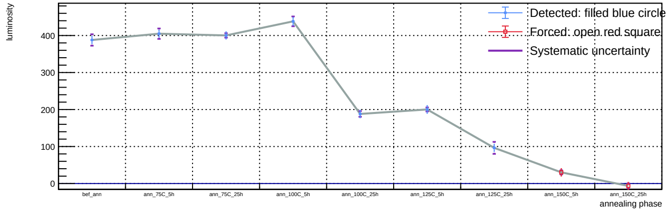
Sensor A1, T = 20 C, representative v = 58.3 V (max available) - Spot 10: luminosity vs phase
