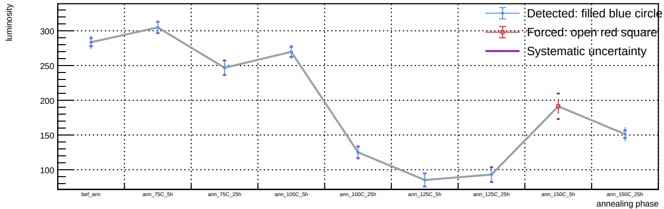
Sensor A1, T = 20 C, representative v = 58.3 V (max available) - Spot 12: luminosity vs phase
