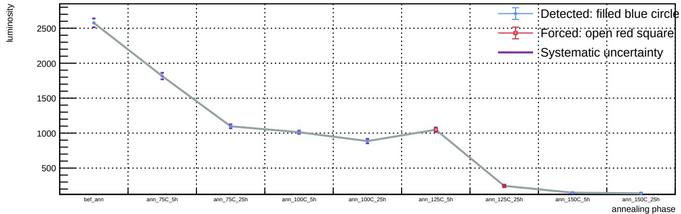
Sensor A1, T = 20 C, representative v = 58.3 V (max available) - Spot 13: luminosity vs phase
