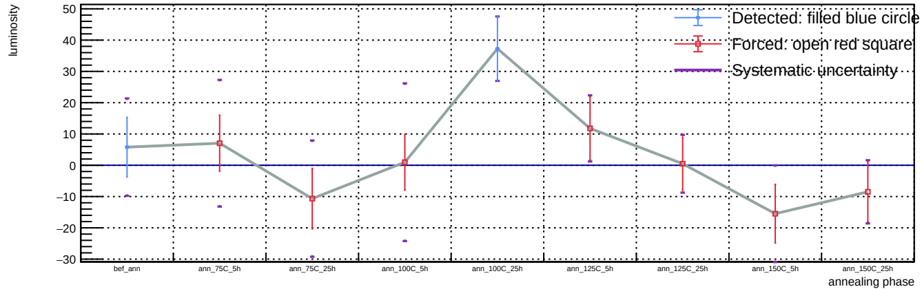
Sensor A1, T = 20 C, representative v = 58.3 V (max available) - Spot 52: luminosity vs phase
