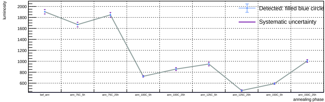
Sensor A1, T = 20 C, representative v = 58.3 V (max available) - Spot 6: luminosity vs phase
