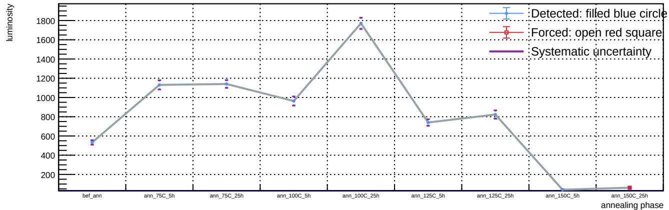
Sensor A1, T = 20 C, representative v = 58.3 V (max available) - Spot 7: luminosity vs phase
