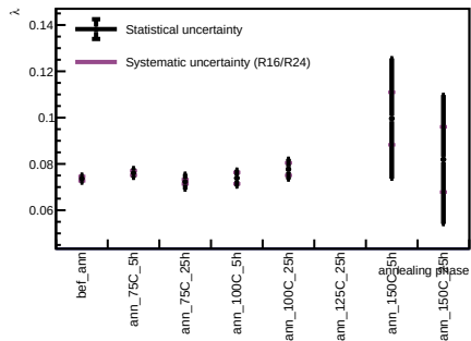
Sensor A1, v = 5 V - Spot 13
