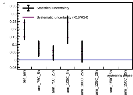
Sensor A1, v = 5 V - Spot 16
