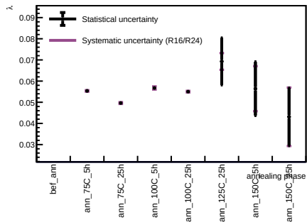
Sensor A1, v = 5 V - Spot 54
