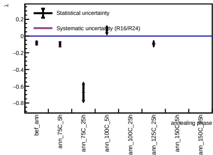
Sensor A1, v = 5 V - Spot 58
