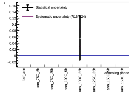
Sensor A1, v = 5 V - Spot 76
