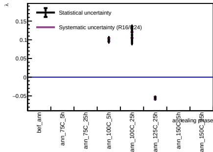
Sensor A1, v = 5 V - Spot 73
