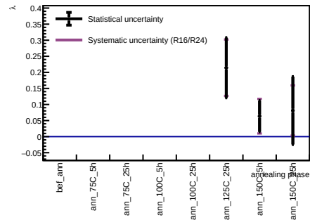
Sensor A1, v = 5 V - Spot 86
