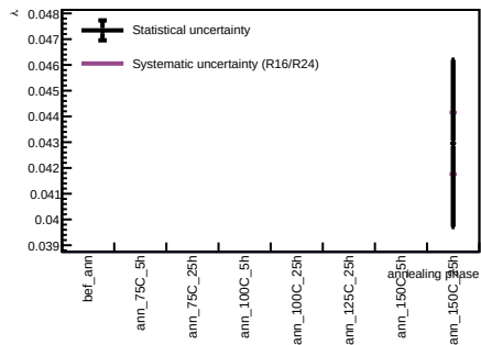
Sensor A1, v = 5 \text{ V} - Spot 88
