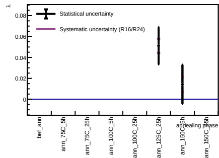
Sensor A1, v = 5 V - Spot 87
