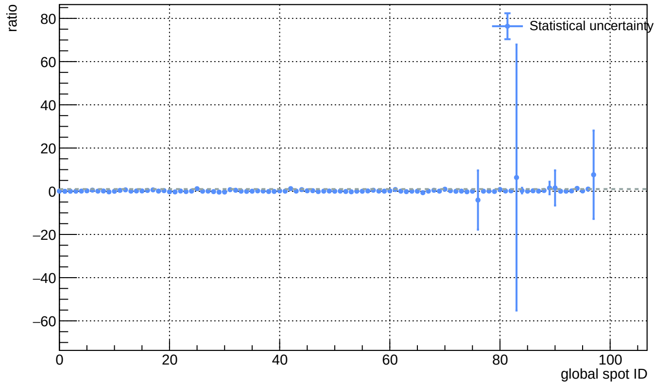
Sensor A1, v = 5 \text{ V} - L(\text{ann } 150^\circ\text{C } 25\text{h}) / L(\text{before annealing})
