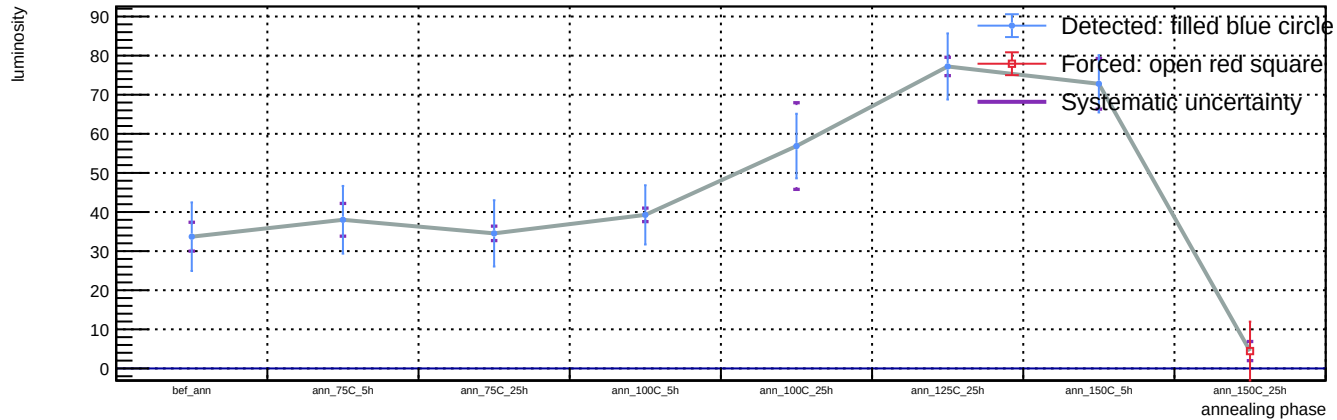
Sensor A1, v = 5 V, representative T = 23 C (max available) - Spot 14: luminosity vs phase
