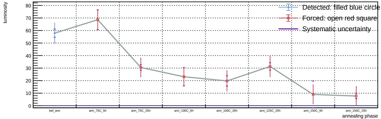
Sensor A1, v = 5 V, representative T = 23 C (max available) - Spot 15: luminosity vs phase
