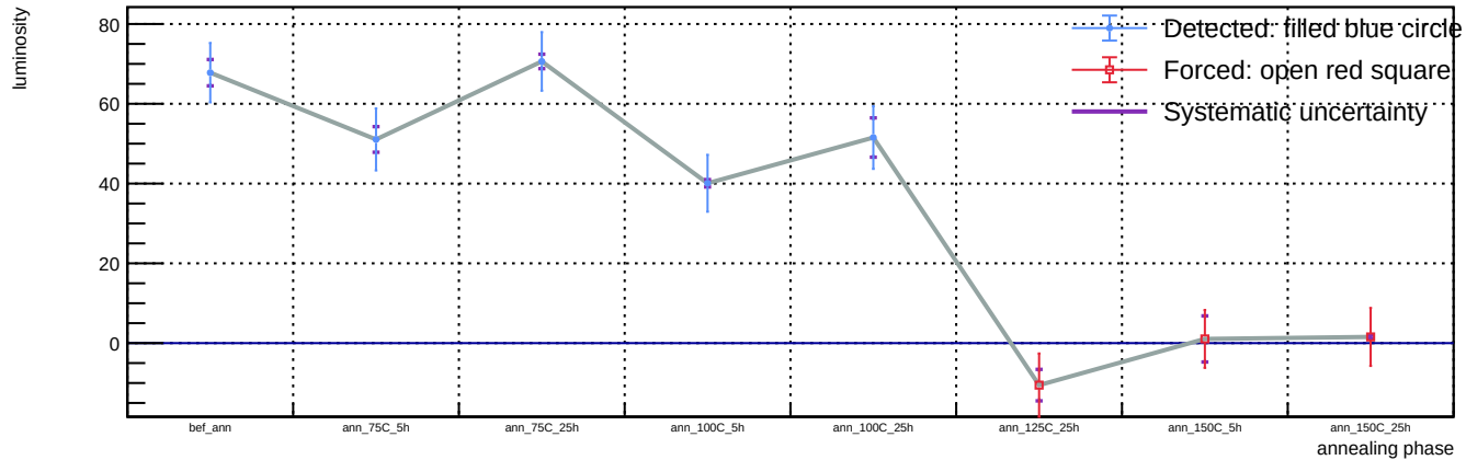
Sensor A1, v = 5 V, representative T = 23 C (max available) - Spot 26: luminosity vs phase
