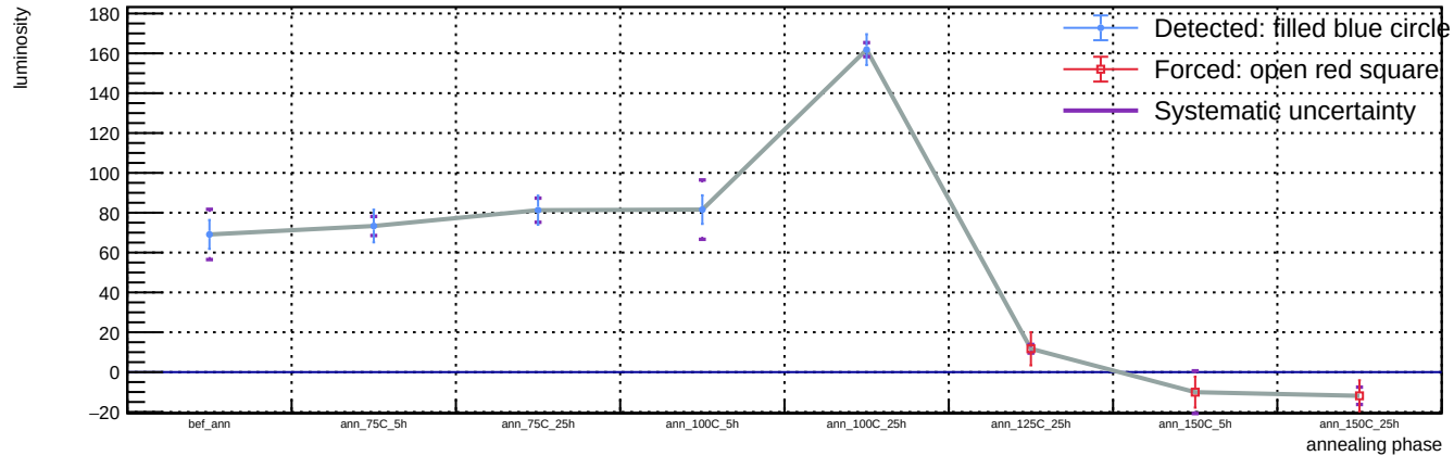
Sensor A1, v = 5 V, representative T = 23 C (max available) - Spot 28: luminosity vs phase
