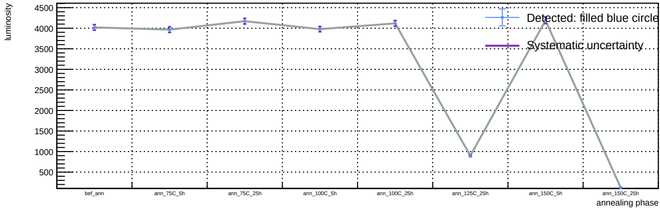
Sensor A1, v = 5 V, representative T = 23 C (max available) - Spot 33: luminosity vs phase
