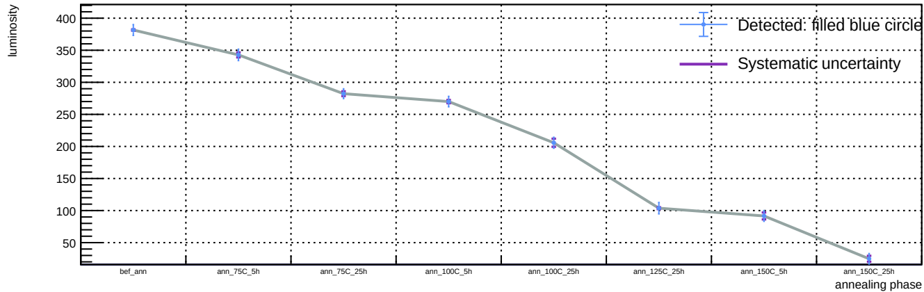
Sensor A1, v = 5 V, representative T = 23 C (max available) - Spot 4: luminosity vs phase
