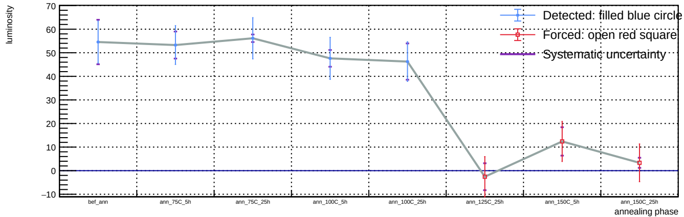
Sensor A1, v = 5 V, representative T = 23 C (max available) - Spot 43: luminosity vs phase
