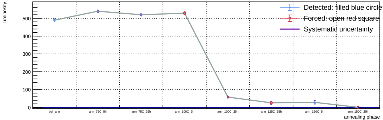
Sensor A1, v = 5 V, representative T = 23 C (max available) - Spot 55: luminosity vs phase
