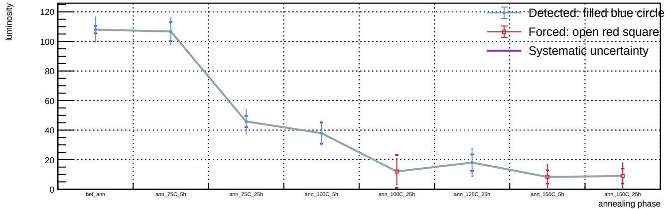
Sensor A1, v = 5 V, representative T = 23 C (max available) - Spot 58: luminosity vs phase
