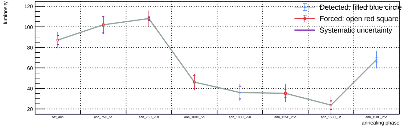
Sensor A1, v = 5 V, representative T = 23 C (max available) - Spot 61: luminosity vs phase
