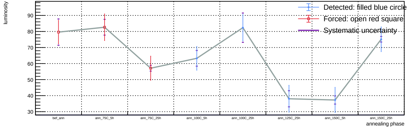
Sensor A1, v = 5 V, representative T = 23 C (max available) - Spot 70: luminosity vs phase
