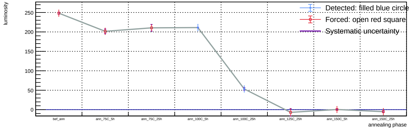
Sensor A1, v = 5 V, representative T = 23 C (max available) - Spot 72: luminosity vs phase
