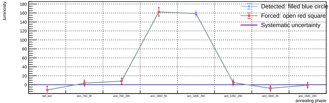
Sensor A1, v = 5 V, representative T = 23 C (max available) - Spot 78: luminosity vs phase
