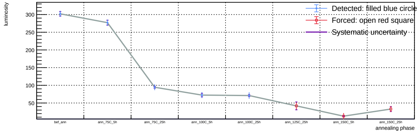
Sensor A1, v = 5 V, representative T = 23 C (max available) - Spot 8: luminosity vs phase
