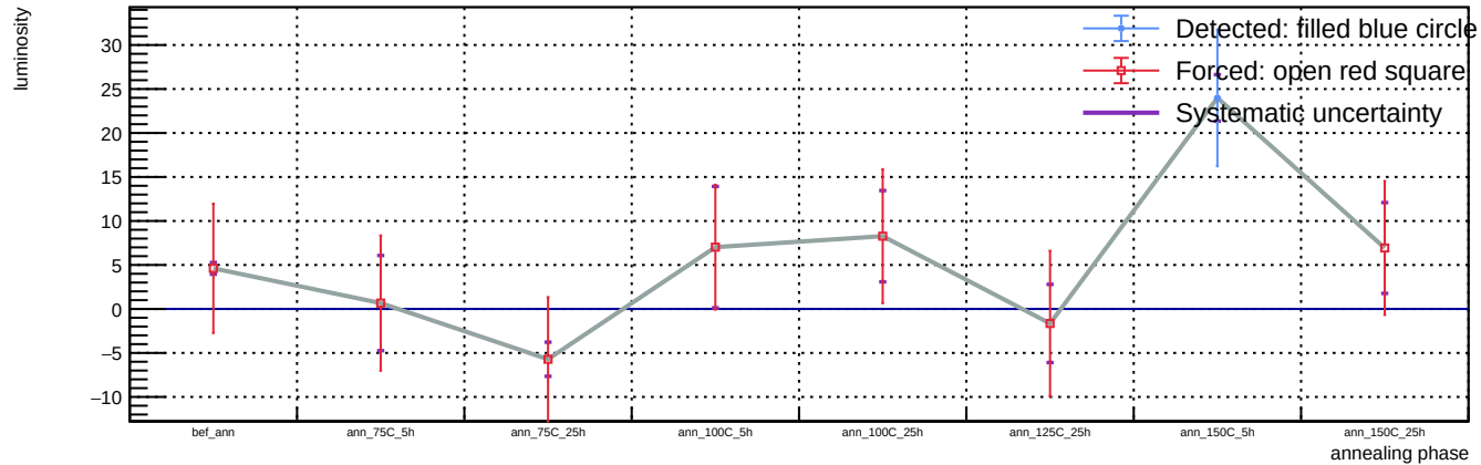
Sensor A1, v = 5 V, representative T = 23 C (max available) - Spot 89: luminosity vs phase
