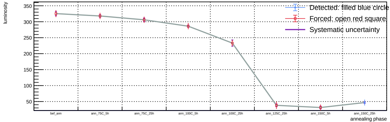
Sensor A1, v = 5 V, representative T = 23 C (max available) - Spot 95: luminosity vs phase
