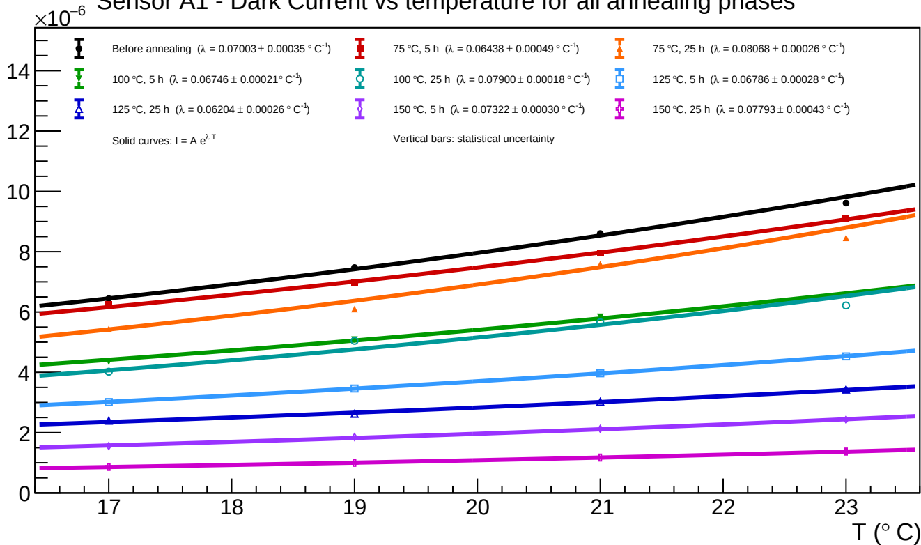
Sensor A1 - Dark Current vs temperature for all annealing phases
