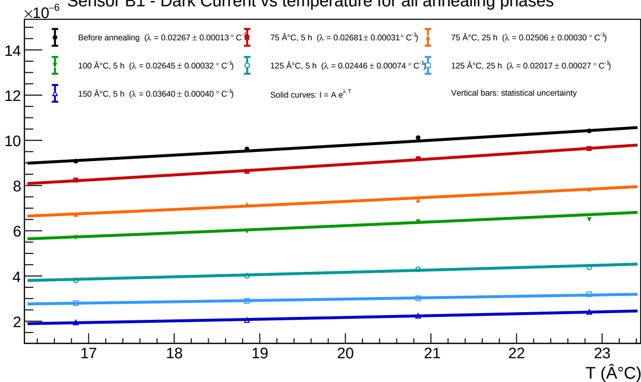
Sensor B1 - Dark Current vs temperature for all annealing phases
