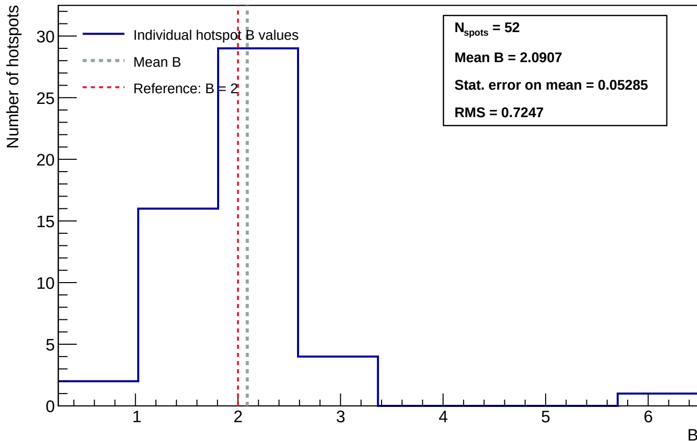
Sensor A1 - Distribution of power-law exponent B - annealing_T=100_h=25
