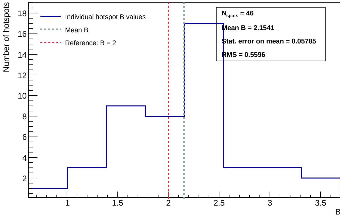
Sensor A1 - Distribution of power-law exponent B - annealing_T=100_h=5
