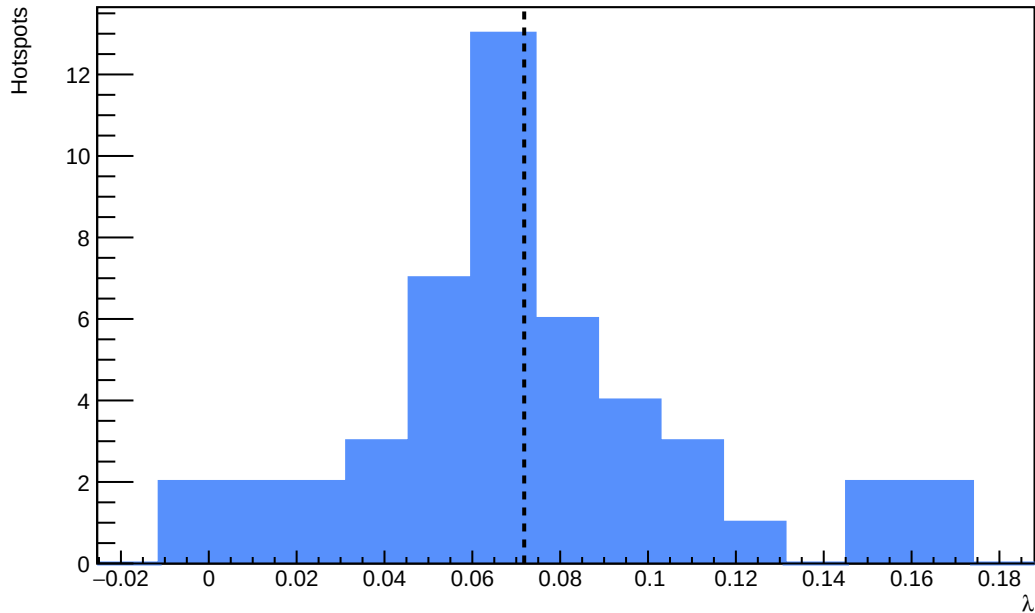
A1_v=5_annealing_T=75_h=25 - Distribution of fitted \lambda - annealing_T=75_h=25
