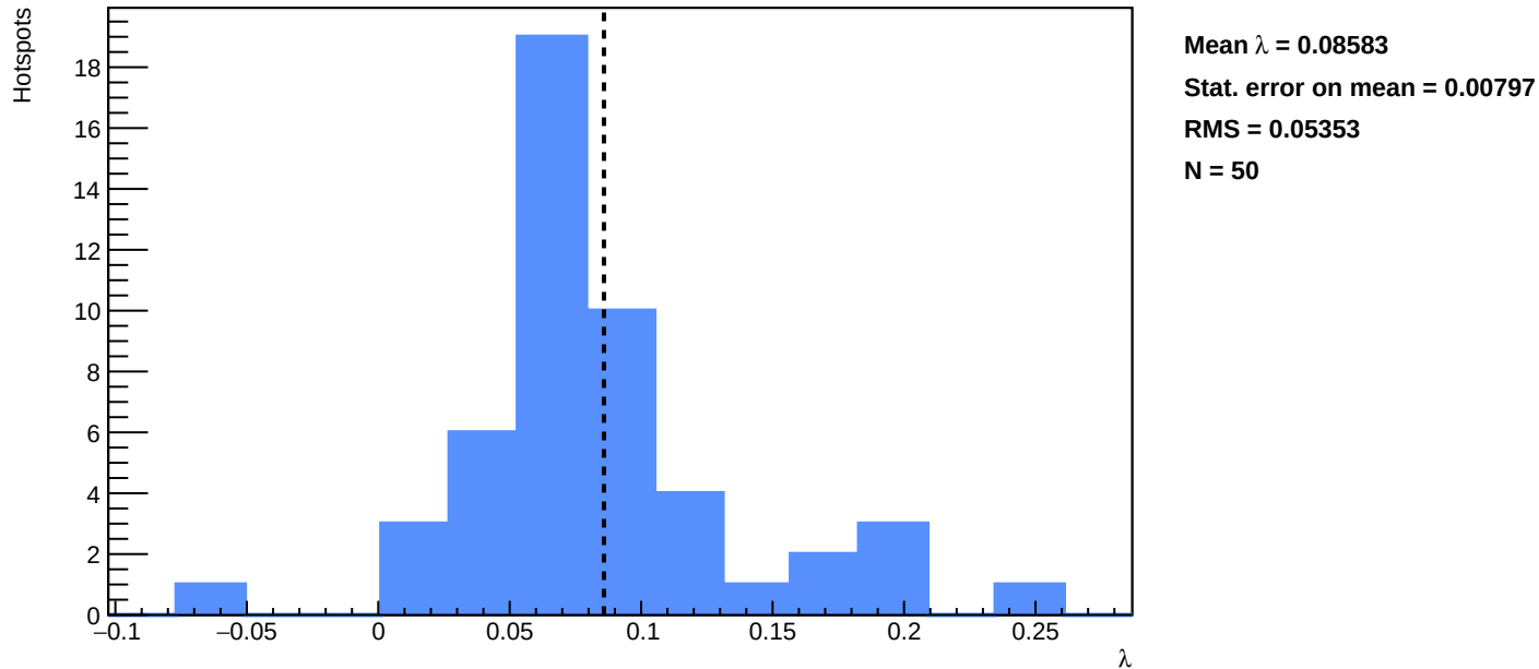
A1_v=5_before_annealing - Distribution of fitted \lambda - before_annealing
