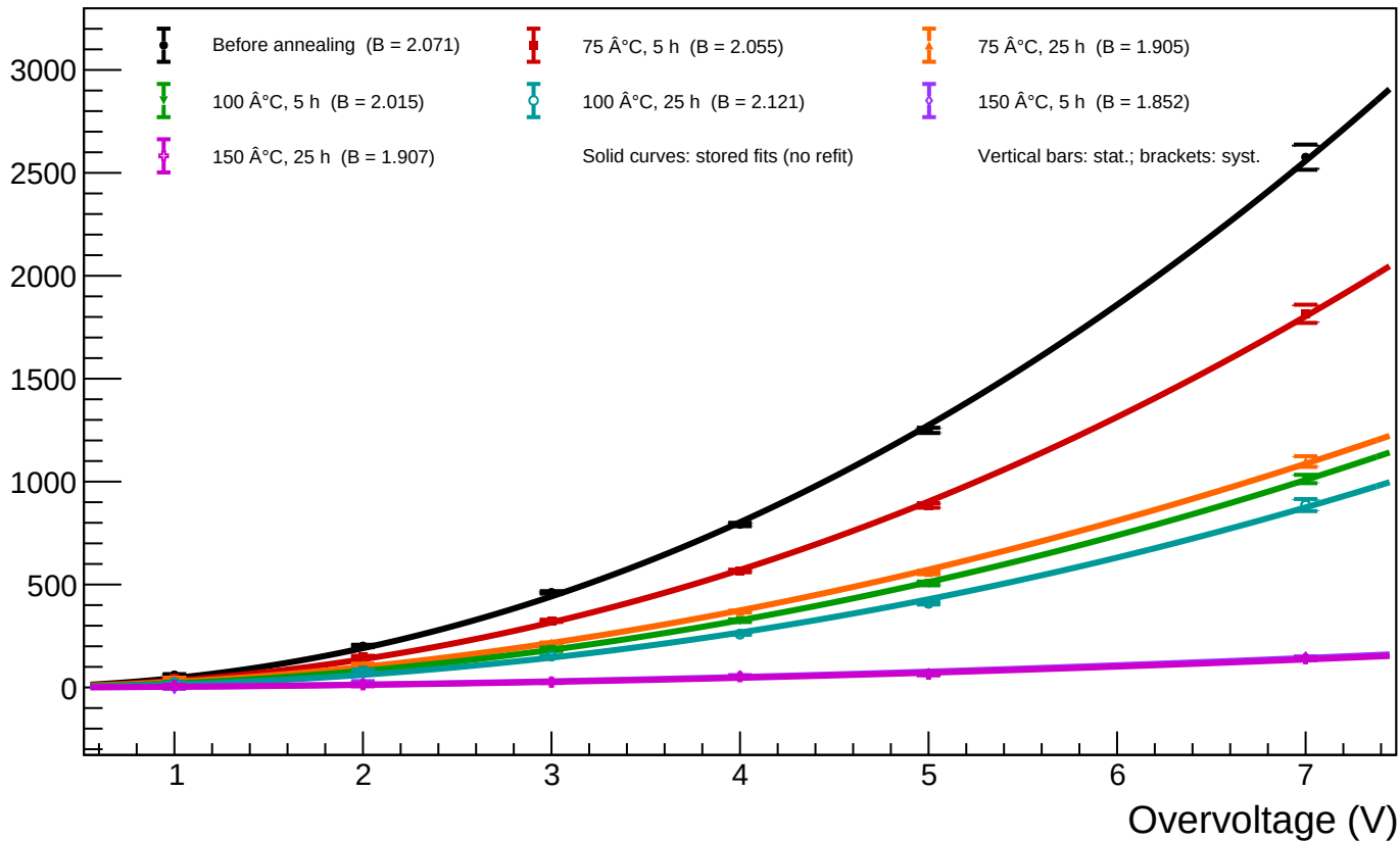
A1_T=20 - Spot 13 ( x = 429.64 , y = 487.00 ): luminosity vs overvoltage for all annealing phases
