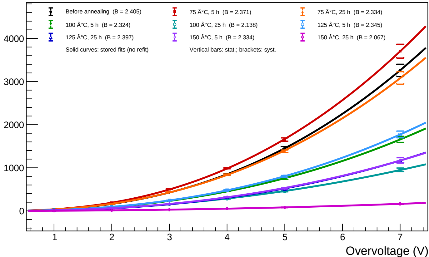
A1 T=20 - Spot 18 (x = 649.85, y = 574.01): luminosity vs overvoltage for all annealing phases
