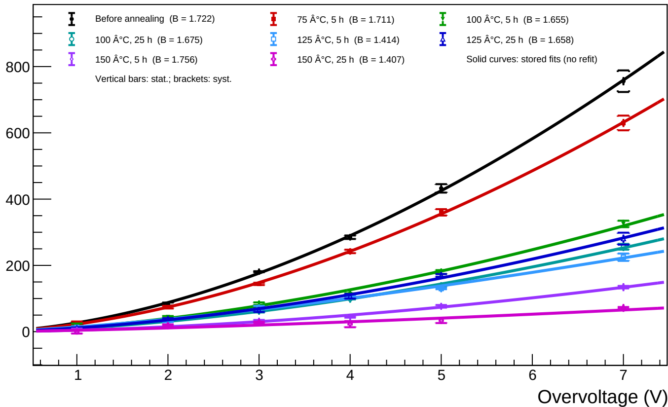
A1_T=20 - Spot 22 ( x = 808.13 , y = 587.46 ): luminosity vs overvoltage for all annealing phases
