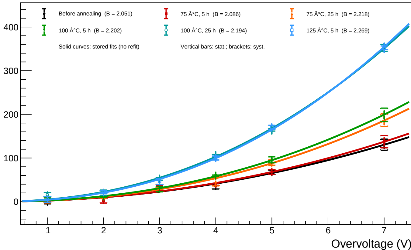
A1_T=20 - Spot 23 ( x = 816.45 , y = 315.29 ): luminosity vs overvoltage for all annealing phases
