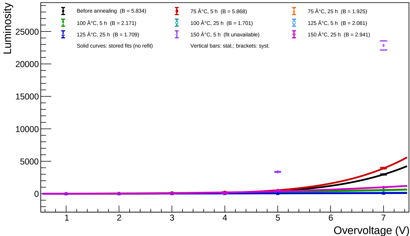
A1_T=20 - Spot 24 (x = 868.58, y = 1007.50): luminosity vs overvoltage for all annealing phases
