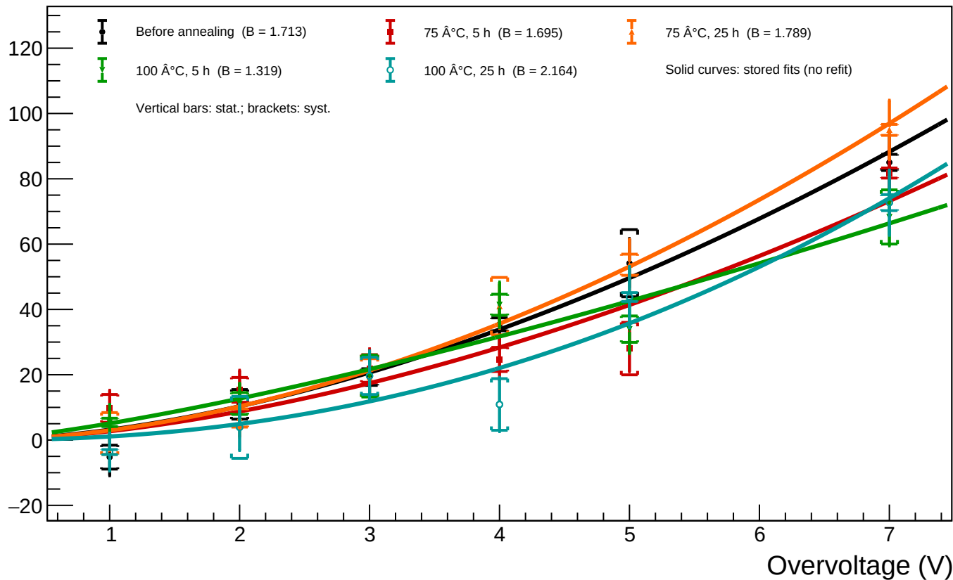
A1_T=20 - Spot 26 (x = 1006.88, y = 123.26): luminosity vs overvoltage for all annealing phases
